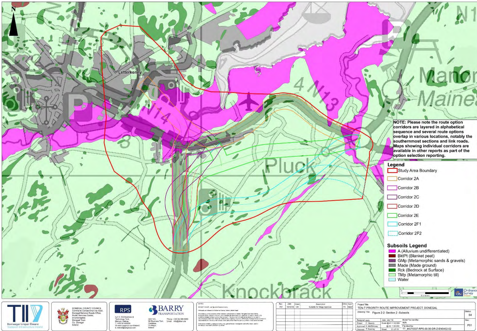
Figure 2-2: Subsoils
