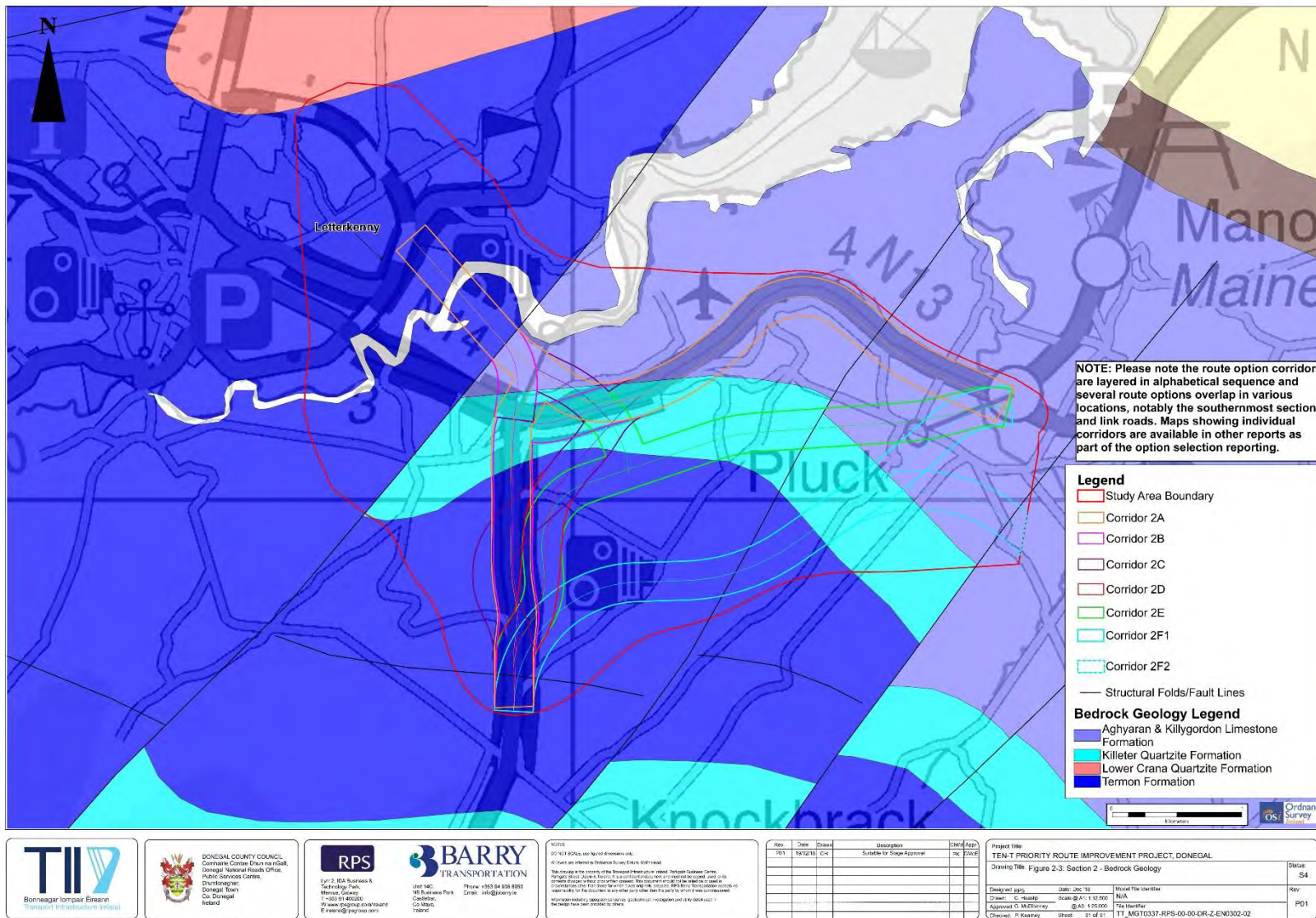
Figure 2-3: Bedrock Geology
