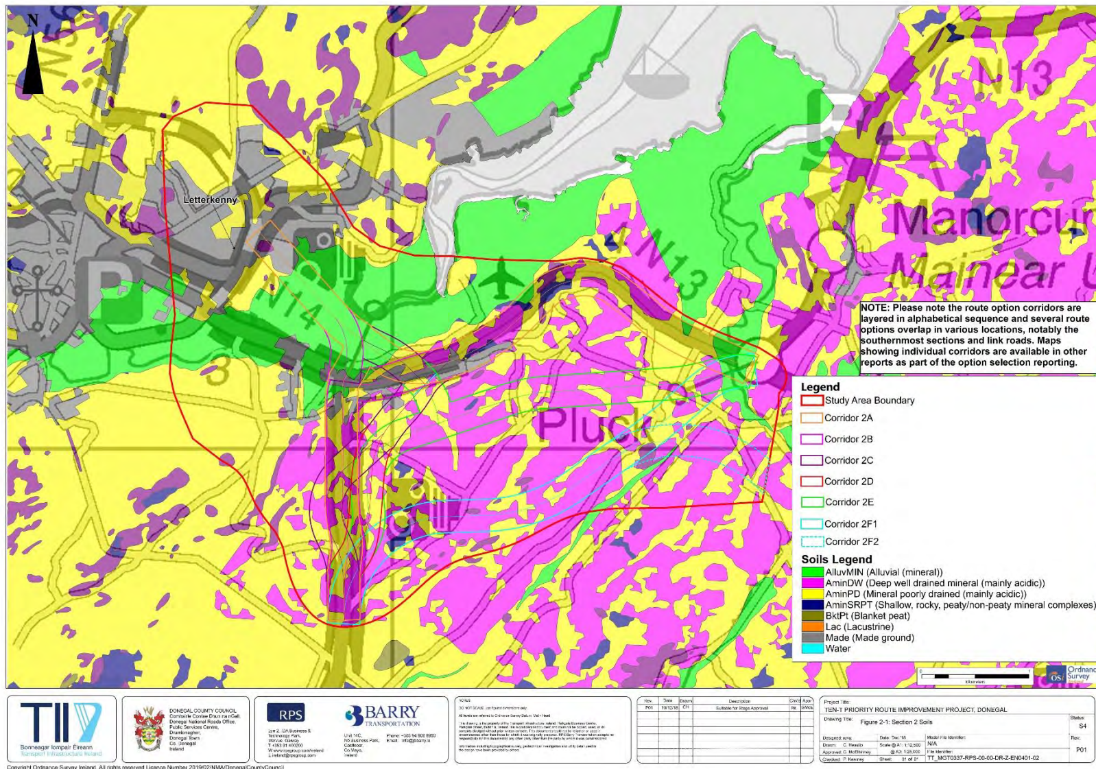
Figure 2-1: Soils
