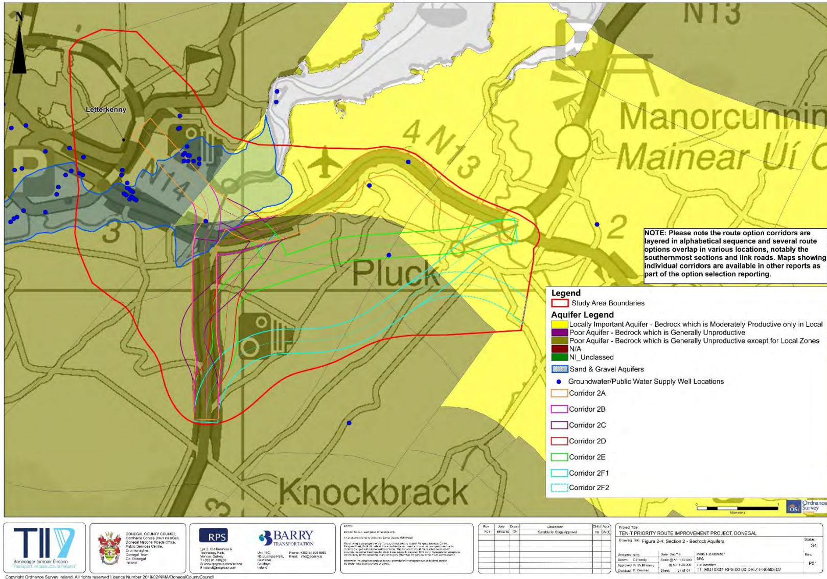
Figure 2-4: Bedrock Aquifers
