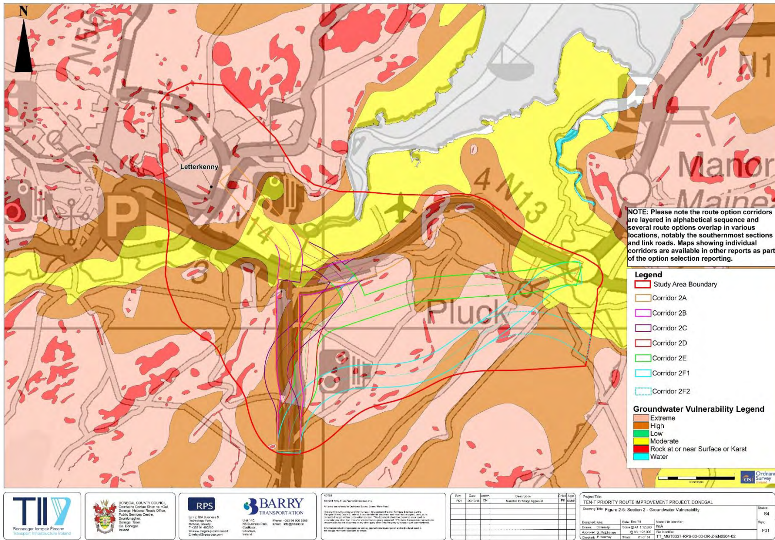
Figure 2-5: Groundwater vulnerability
